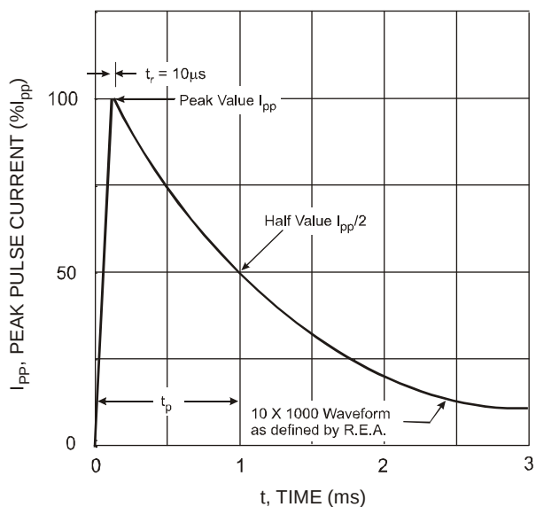
Fig. 4 Pulse Waveform
