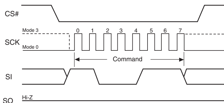
Figure 9.10 Bulk Erase (BE) Command Sequence
